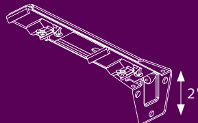
6" Double Wall Bracket with Wide Base adjusts 2 1/2" - 4" and 6" - 7 1/2"
