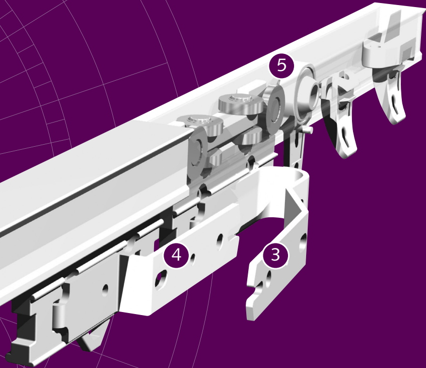
3" Wall Bracket with Wide Base adjusts 3" - 4 1/2"
