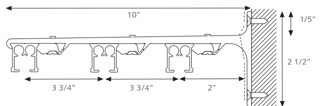
Smart Klick Triple Wall Bracket
