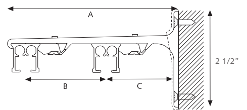
Smart Klick Triple Wall Bracket
