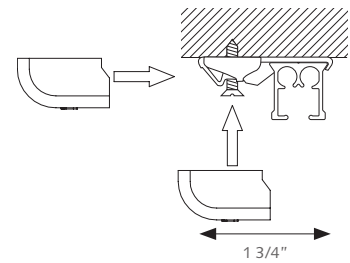
Smart Klick Ceiling Bracket with cover
