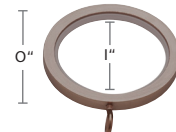
3035RIN-XX 1 3/8" Flat Ring w/ Plastic Insert O: 2 1/2" I: 1 7/8" 3045RIN-XX 1 3/4" Flat Ring w/ Plastic Insert O: 2 3/8" I: 2"
