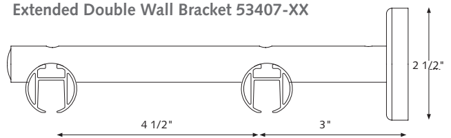
Extended Double Wall Bracket 53407-XX
